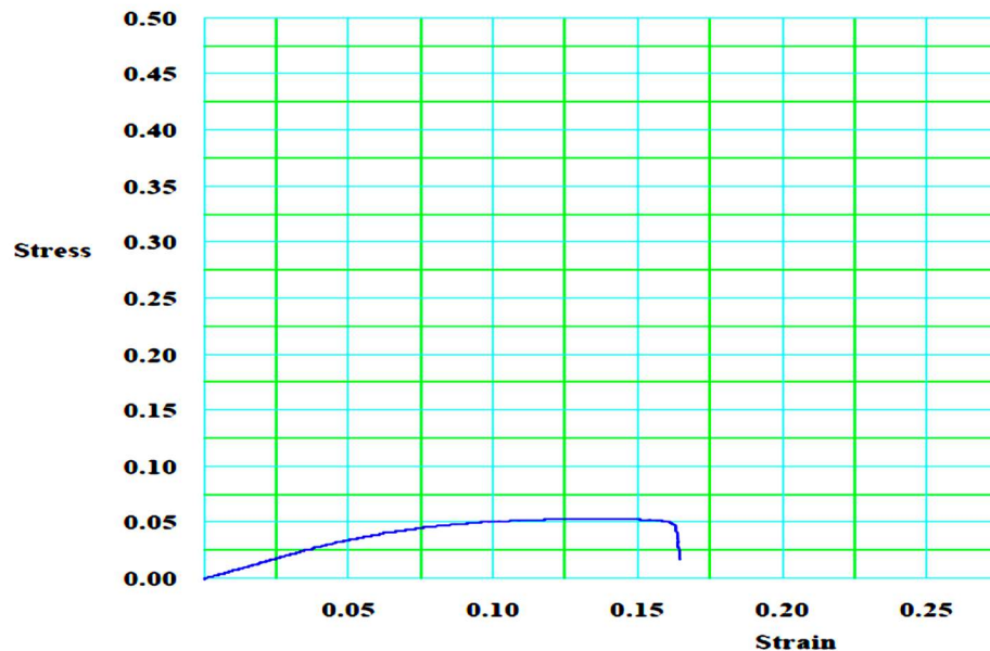
Figure4: Stress-Strain analysis of wood flour-pp composite
