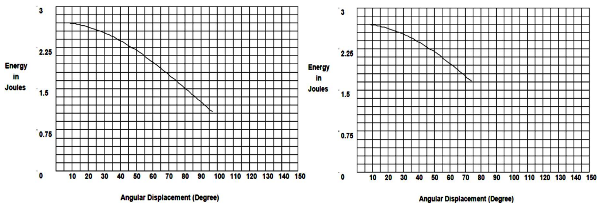
Figure2: Impact test Characteristics of wood flour-pp and jute-pp composite.
