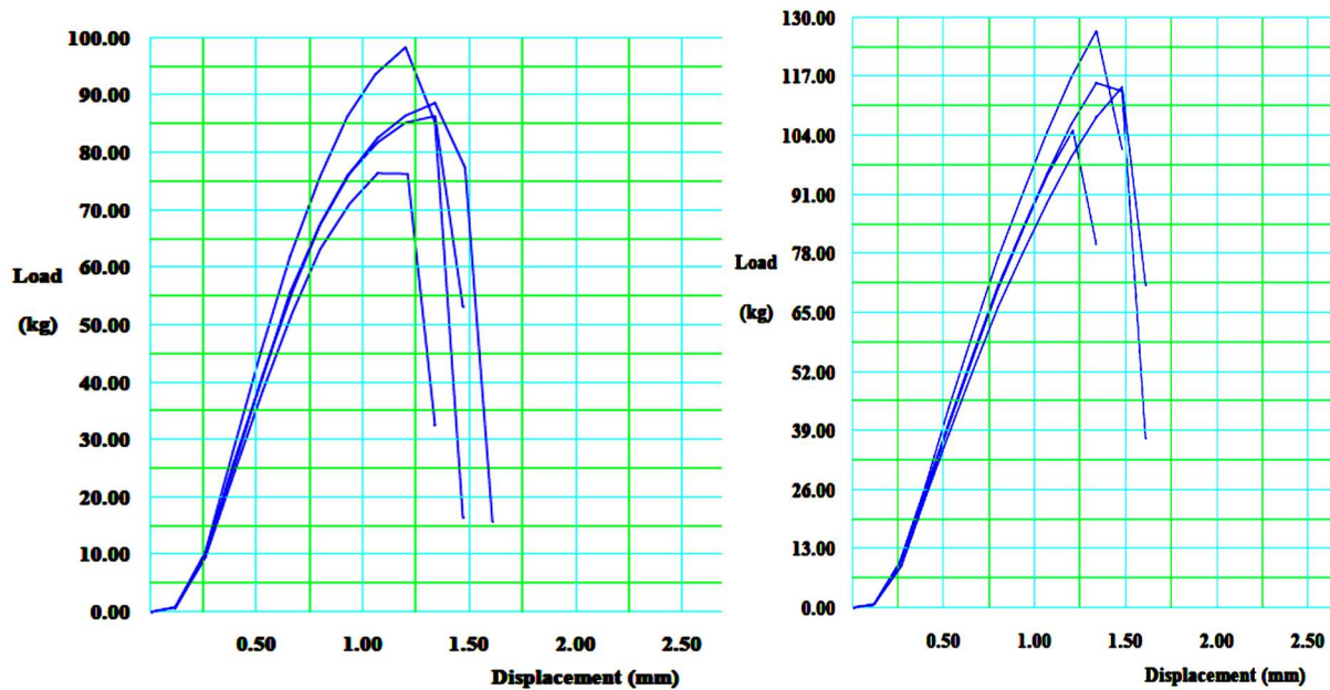
Figure1: Tensile Characteristics of wood flour-pp and jute-pp composite.
