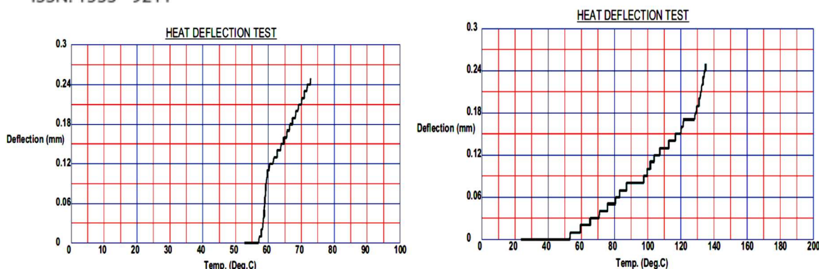
Figure5: HDT testing of wood flour-pp & jute-pp composite
