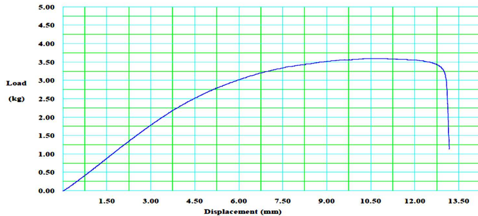
Figure3: Load-Displacement characteristics for wood flour-pp composite
